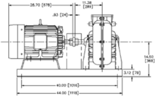
TurboPak VFD
