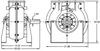
TurboTron Regenerative Blower/Exhauster
